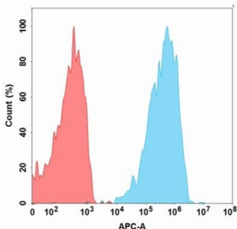
Figure 1. Flow cytometry analysis with 15 \mu\text{g}/\text{mL} CXCR4 (ulocuplumab biosimilar) mAb (28101) on Expi293 cells transfected with Human CXCR4 protein (Blue histogram) or Expi293 transfected with irrelevant protein (Red histogram).
