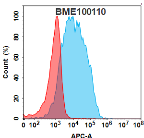
Figure 1. Flow cytometry analysis with 15µg/mL TLR2(tomaralimab biosimilar) mAb (28109) on Expi293 cells transfected with Human TLR2 protein (Blue histogram) or Expi293 transfected with irrelevant protein (Red histogram).
