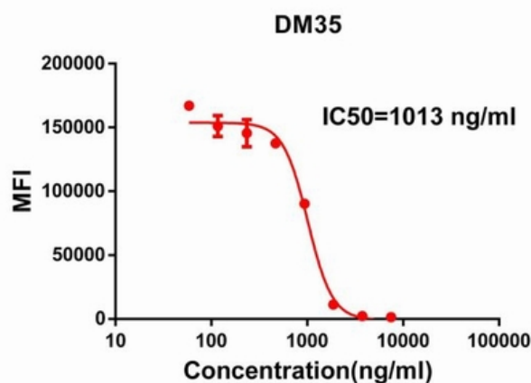
Figure 2. Competition flow cytometry assay demonstrating Rabbit RBD monoclonal antibody ( clone: DM35) blockade of SARS-CoV-2 (COVID-19) S protein RBD (1 µg/ml, [getskuurl sku=11301 binding to Expi 293 cell line transfected with human ACE2. IC50=1013ng/ml. The Y-axis represents the geometric mean fluorescence intensity (MFI) while the X-axis represents the concentration of IgG used.
