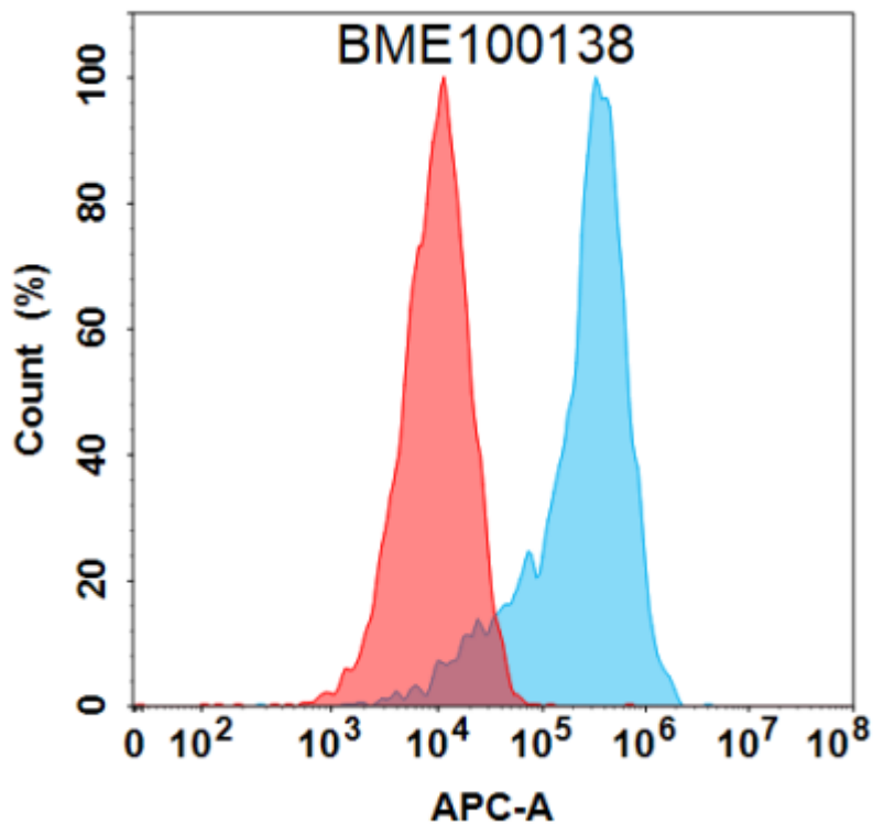
Figure 1. Flow cytometry analysis with 1 \mu g/mL TFRC mAb (28132) on Expi293 cells transfected with Human TFRC protein (Blue histogram) or Expi293 transfected with irrelevant protein (Red histogram).
