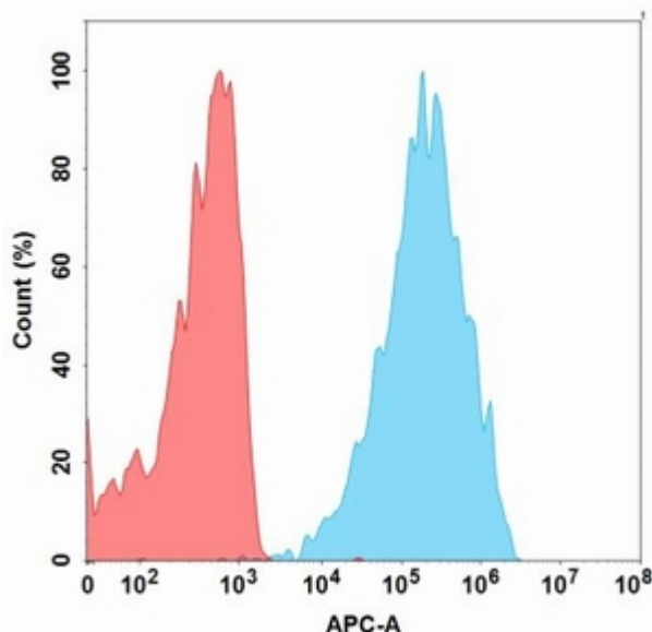
Figure 1. Flow cytometry analysis with 1 \mu\text{g}/\text{mL} NKG2A (monalizumab biosimilar) mAb (28088) on Expi293 cells transfected with Human NKG2A protein and Human CD94 protein (Blue histogram) or Expi293 transfected with irrelevant protein (Red histogram).
