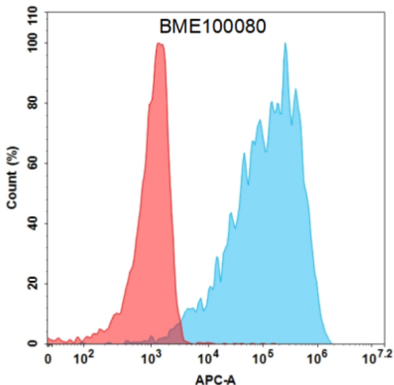
Figure 1. Flow cytometry analysis with TSHR(K1-70) mAb 15 \mu g/mL on Expi293 cells transfected with Human TSHR (Blue histogram) or Expi293 transfected with irrelevant protein (Red histogram).
