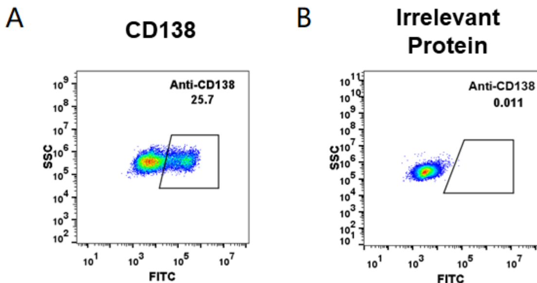
Figure 1. HEK293 cell line transfected with irrelevant protein (B) and human CD138 (A) were surface stained with CD138 neutralizing antibody 1\mu\text{g}/\text{ml} (indatuximab) followed by Alexa 488-conjugated human IgG secondary antibody.
