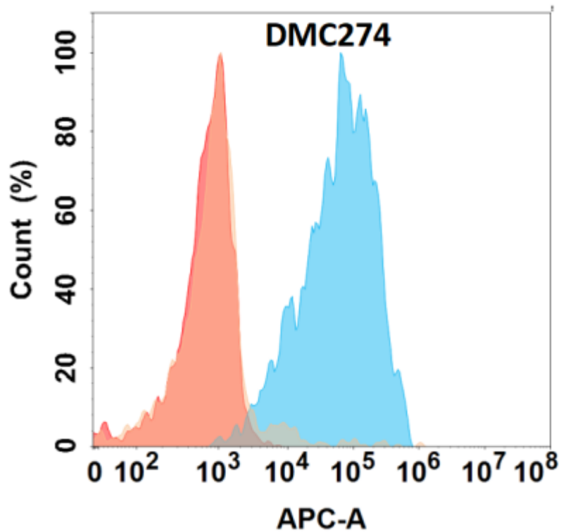
Figure 1. Flow cytometry analysis with IL5 (DMC274) on Expi293 cells transfected with human IL5 (Blue histogram) or Expi293 transfected with irrelevant protein (Red histogram).
