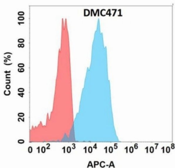
Figure 1. Flow cytometry analysis with IL22 (DMC471) on Expi293 cells transfected with human IL22 (Blue histogram) or Expi293 transfected with irrelevant protein (Red histogram)
