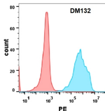
Figure 2. Flow cytometry analysis with HVEM (DM132) on Expi293 cells transfected with human HVEM (Blue histogram) or Expi293 transfected with irrelevant protein (Red histogram).
