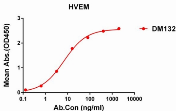
Figure 1. ELISA plate pre-coated by 1 µg/ml (100 µl/well) Human HVEM protein, His tagged protein 11253 can bind Rabbit HVEM monoclonal antibody (clone: DM132) in a linear range of 0.1-12 ng/ml.
