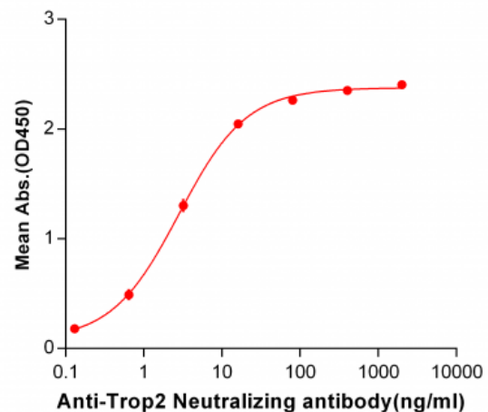
Figure 2. ELISA plate pre-coated by 2 µg/ml (100 µl/well) Human Trop2, mFc-His tagged protein (11304) can bind Trop2 Neutralizing antibody 28032 in a linear range of 0.13-16.0 ng/ml.
