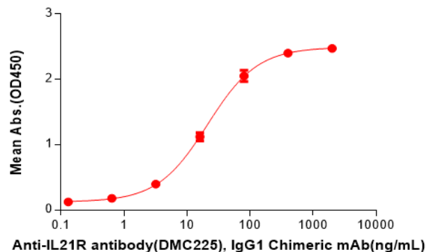
Figure 2. ELISA plate pre-coated by 2 µg/ml (100 µl/well) Human IL21R Protein, mFc Tag(11383) can bind IL21R antibody(DMC225), IgG1 Chimeric mAb in a linear range of 3.20-80 ng/mL.
