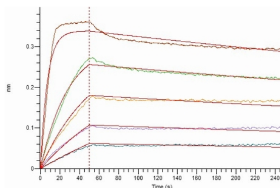
Figure 2. Loaded Human IL-2RA-Fc on Protein A Biosensor, can bind Human IL-2 Superkine with an affinity constant of 0.58 nM as determined in BLI assay.
