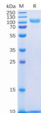
Figure 1. Human HER3 Protein, His Tag on SDS-PAGE under reducing condition.
