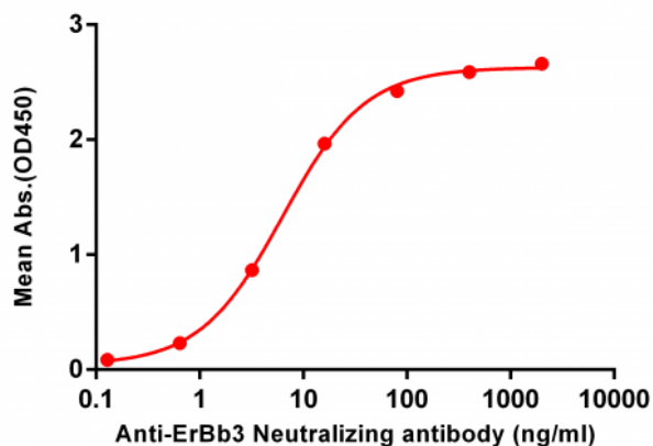
Figure 3. ELISA plate pre-coated by 1 \mu g/ml (100 \mu l/well) Human Her3, His tagged protein (11208) can bind ErBb3 Neutralizing antibody 28065 in a linear range of 3.2-16 ng/ml.
