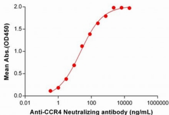
Figure 2. ELISA plate pre-coated by 2 \mu g/ml (100 \mu l/well) Human CCR4(1-39) Protein, hFc Tag (11605) can bind CCR4 Neutralizing antibody 28089 in a linear range of 1.02-740.74 ng/mL.
