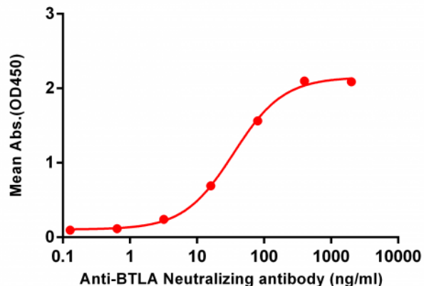
Figure 2. ELISA plate pre-coated by 1 \mu g/ml (100 \mu l/well) Human BTLA, His tagged protein (11324) can bind BTLA Neutralizing antibody 28062 in a linear range of 16-80 ng/ml.
