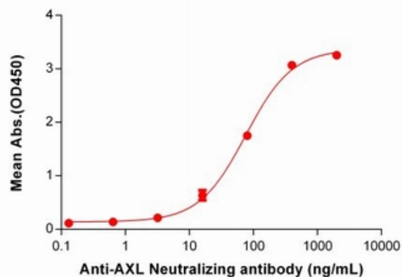
Figure 2. ELISA plate pre-coated by 1 \mu g/ml (100 \mu l/well) Human AXL, hFc tagged protein (11332) can bind AXL Neutralizing Antibody 28042 in a linear range of 0.64–80.0 ng/ml.
