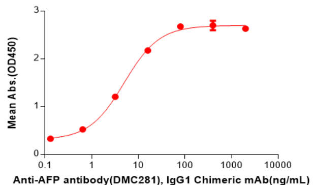
Figure 2. ELISA plate pre-coated by 2 µg/ml (100 µl/well) Human AFP Protein, hFc Tag(11198) can bind AFP antibody(DMC281), IgG1 Chimeric mAb in a linear range of 0.64-16 ng/mL.
