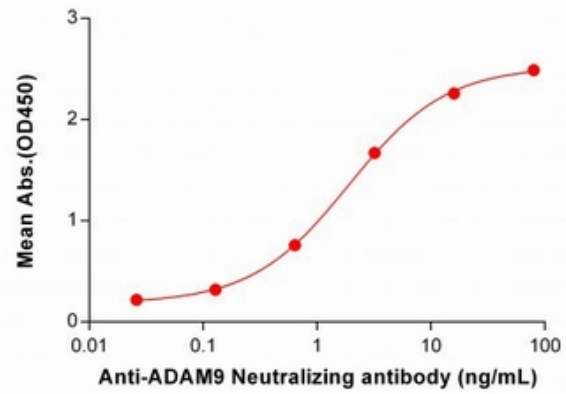
Figure 2. ELISA plate pre-coated by 1 µg/ml (100 µl/well) Human ADAM9 protein, His Tag (11663) can bind ADAM9 Neutralizing antibody 28071 in a linear range of 0.128-16 ng/mL.
