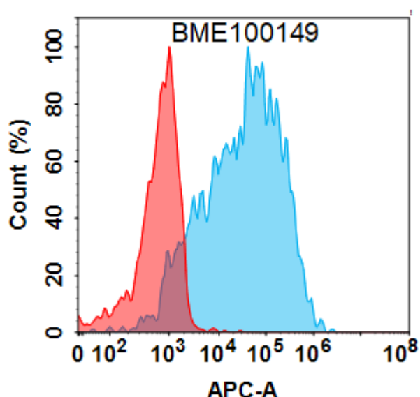
Figure 1. Flow cytometry analysis with 15 µg/mL HTRA1(galegenimab biosimilar) mAb (28141) on Expi293 cells transfected with Human HTRA1 protein (Blue histogram) or Expi293 transfected with irrelevant protein (Red histogram).
