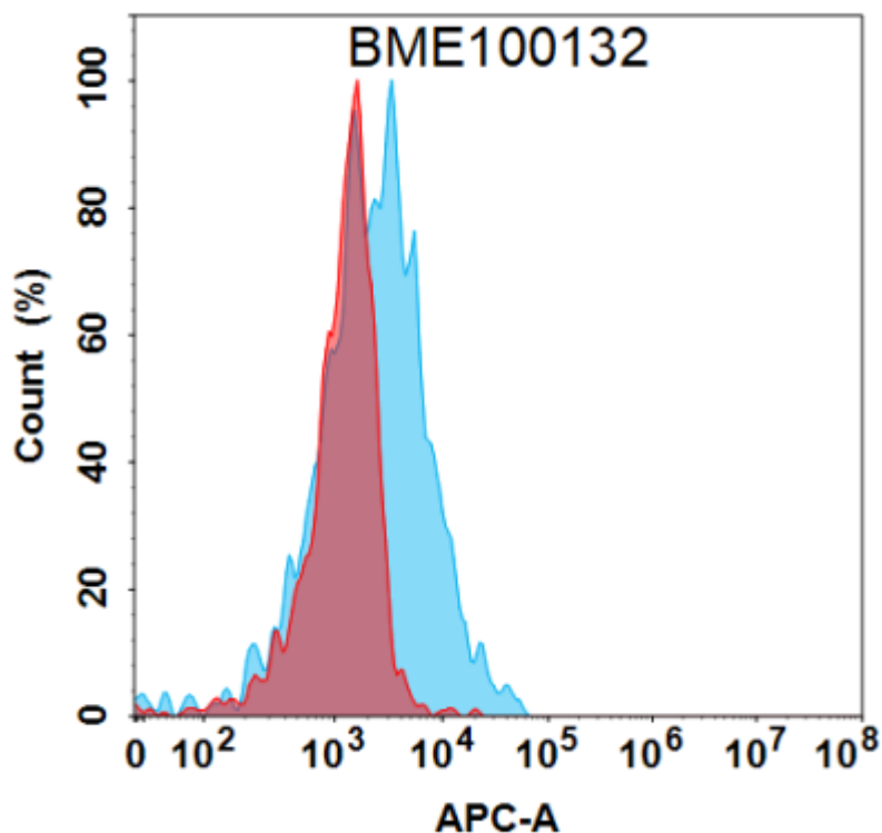
Figure 1. Flow cytometry analysis under cell membrane permeable condition with 1 \mu g/mL IL20 (fletikumab biosimilar) mAb (28127) on Expi293 cells transfected with Human IL20 protein (Blue histogram) or Expi293 transfected with irrelevant protein (Red histogram).
