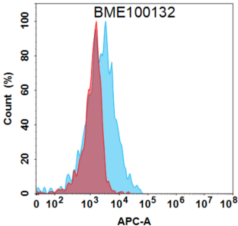
Figure 1. Flow cytometry analysis under cell membrane permeable condition with 1 µg/mL Anti-IL20 (fletikumab biosimilar) mAb (28127) on Expi293 cells transfected with Human IL20 protein (Blue histogram) or Expi293 transfected with irrelevant protein (Red histogram).
