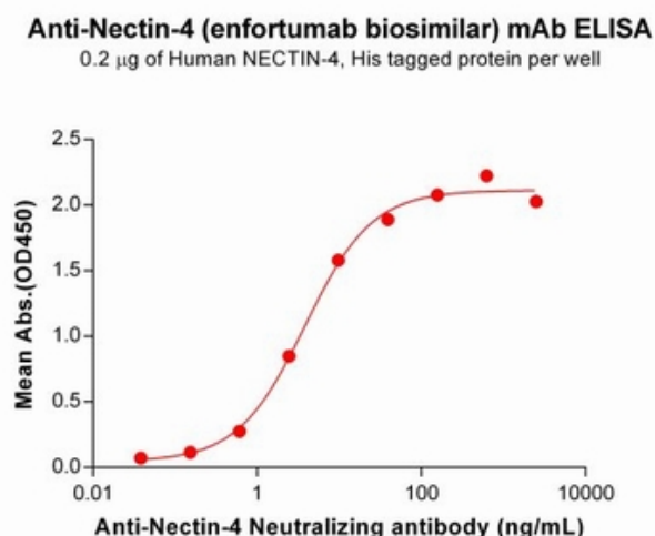
Figure 1. ELISA plate pre-coated by 2 µg/mL (100 µl/well) Human NECTIN-4 Protein, His Tag 11649 can bind Nectin-4 Neutralizing antibody (28091) in a linear range of 0.61-39.06 ng/mL.
