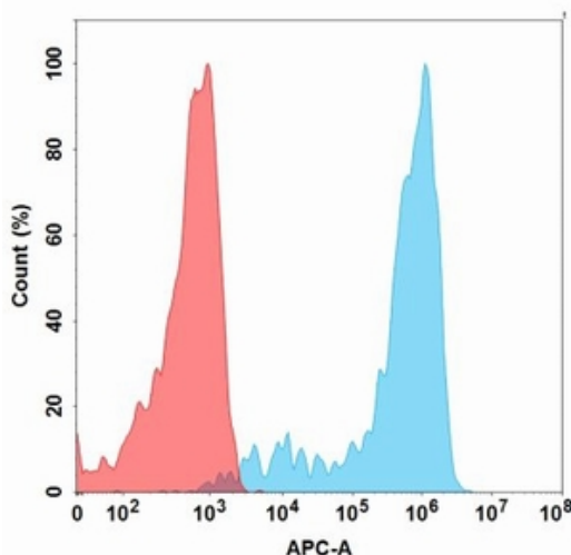
Figure 2. Flow cytometry analysis with 1 µg/mL Nectin-4 (enfortumab biosimilar) mAb (28091) on Expi293 cells transfected with Human Nectin-4 protein (Blue histogram) or Expi293 transfected with irrelevant protein (Red histogram).
