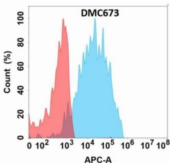
Figure 1. Flow cytometry analysis with CRTAM(DMC673) on Expi293 cells transfected with human CRTAM(Blue histogram) or Expi293 transfected with irrelevant protein (Red histogram).
