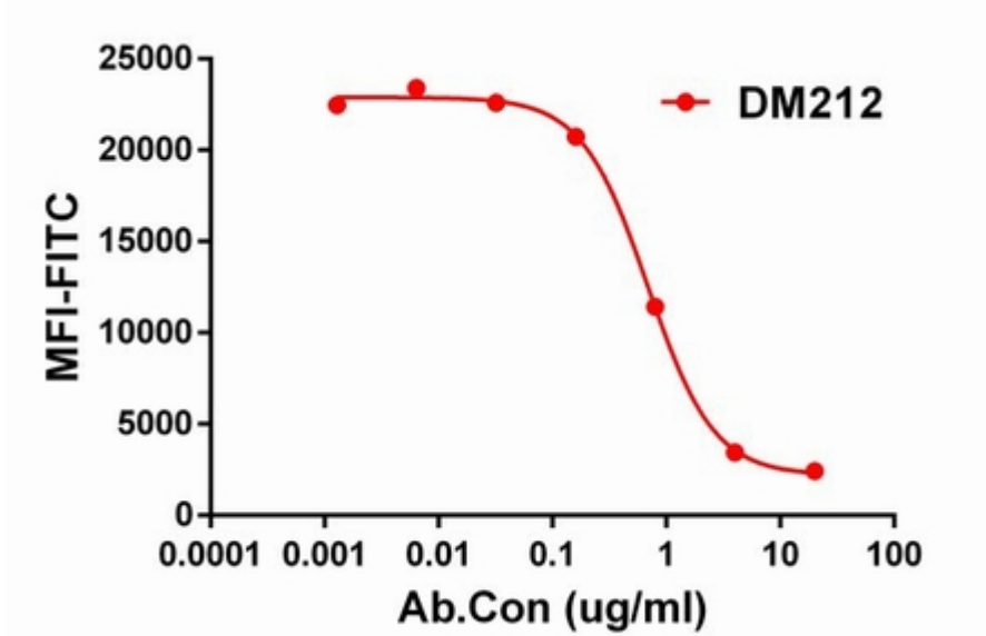
Figure 1. Competition assay demonstrating DM212 blockade of SIRPÎ± binding to Jurkat cell line.
