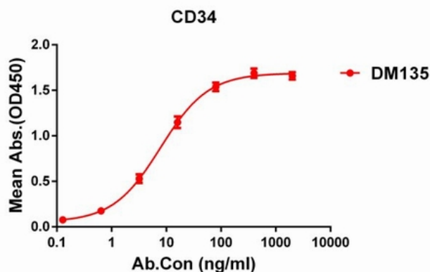
Figure 1. ELISA plate pre-coated by 1 µg/ml (100 µl/well) Human CD34 protein, His tagged protein 11280 can bind Rabbit CD34 monoclonal antibody (clone: DM135) in a linear range of 0.1-12 ng/ml.
