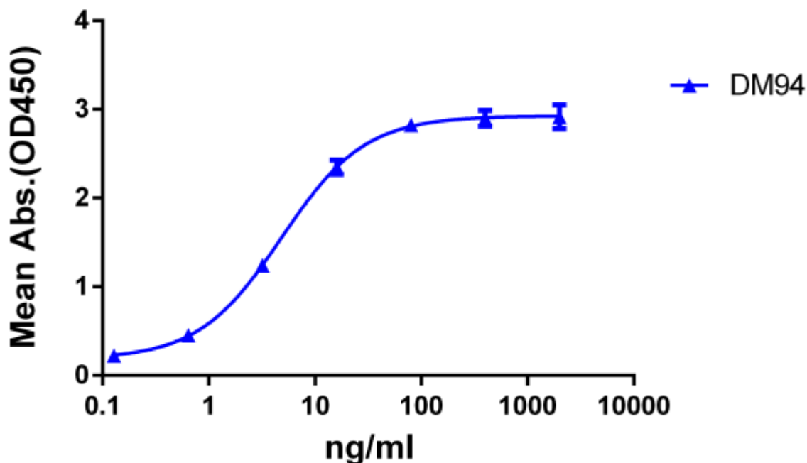
Figure 1. ELISA plate pre-coated by 2 \mu g/ml (100 \mu l/well) Human BTN3A1 protein, mFc-His tagged protein 11180 can bind Rabbit BTN3A1 monoclonal antibody ( clone: DM94) in a linear range of 0.64-80 ng/ml.
