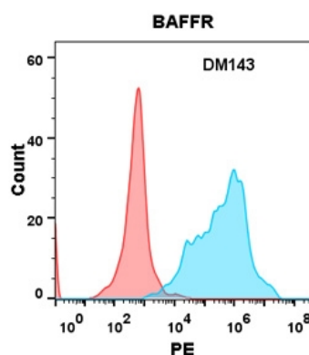
Figure 2. Flow cytometry analysis with BAFFR (DM143) on Expi293 cells transfected with human BAFFR (Blue histogram) or Expi293 transfected with irrelevant protein (Red histogram).
