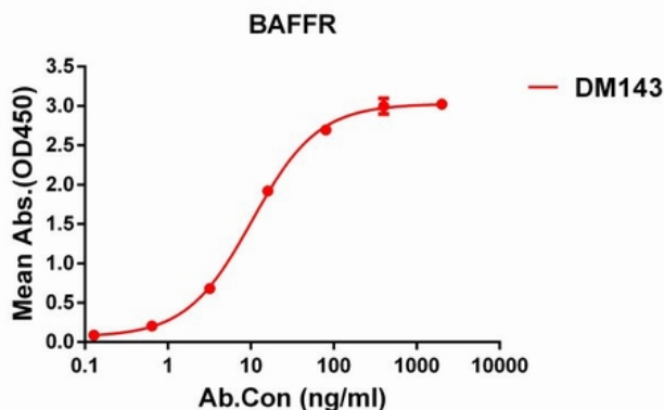
Figure 1. ELISA plate pre-coated by 1 µg/ml (100 µl/well) Human BAFFR protein, mFc tagged protein 11170 can bind Rabbit BAFFR monoclonal antibody (clone: DM143) in a linear range of 0.8-50
