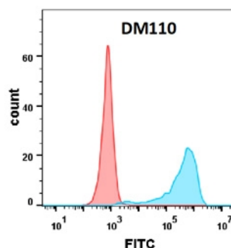
Figure 2. Flow cytometry analysis with B7-1 (DM110) on Expi293 cells transfected with human B7-1 (Blue histogram) or Expi293 transfected with irrelevant protein (Red histogram).
