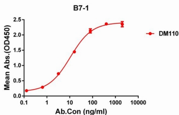
Figure 1. ELISA plate pre-coated by 2 µg/ml (100 µl/well) Human B7-1 protein, hFc tagged protein 11283 can bind Rabbit B7-1 monoclonal antibody (clone: DM110) in a linear range of 0.32-100 ng/ml.
