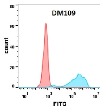
Figure 2. Flow cytometry analysis with B7-1 (DM109) on Expi293 cells transfected with human B7-1 (Blue histogram) or Expi293 transfected with irrelevant protein (Red histogram).
