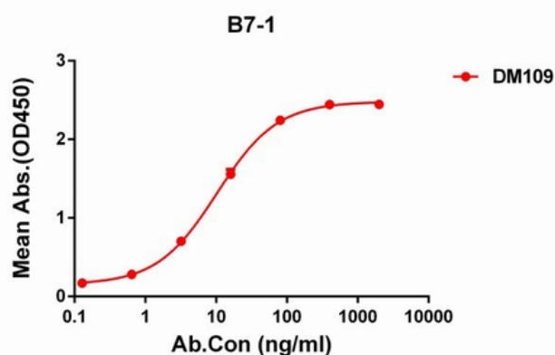
Figure 1. ELISA plate pre-coated by 2 µg/ml (100 µl/well) Human B7-1 protein, hFc tagged protein 11283 can bind Rabbit B7-1 monoclonal antibody (clone: DM109) in a linear range of 0.6-80 ng/ml.
