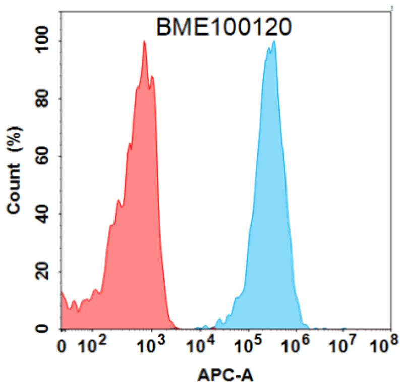
Figure 1. Flow cytometry analysis with 1 \mu\text{g}/\text{mL} C5AR1 (avdoralimab biosimilar) mAb (28118) on Expi293 cells transfected with Human C5AR1 protein (Blue histogram) or Expi293 transfected with irrelevant protein (Red histogram).
