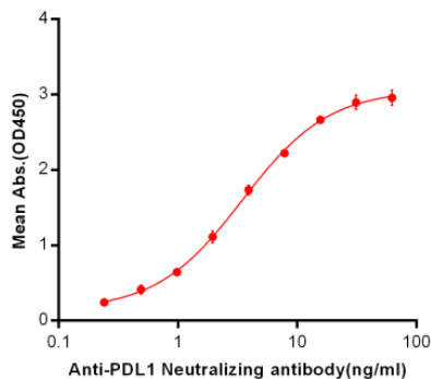
Figure 1. ELISA plate pre-coated by 2 µg/ml (100 µl/well) Human PDL1, mFc-His tagged protein 11151 can bind PDL1 Neutralizing antibody in a linear range of 0.24-7.81 ng/ml.
