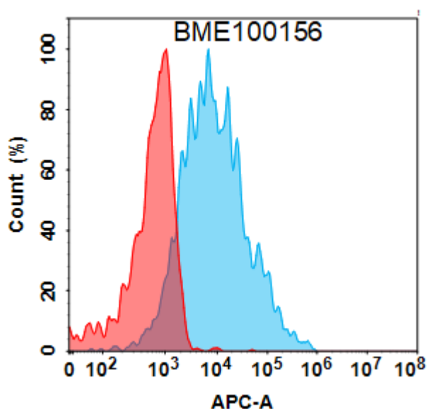
Figure 1. Flow cytometry analysis with 15 µg/mL CD45 (apamistamab biosimilar) mAb (28148) on Expi293 cells transfected with Human CD45 protein (Blue histogram) or Expi293 transfected with irrelevant protein (Red histogram).
