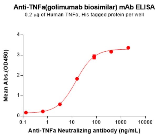
Figure 2. ELISA plate pre-coated by 2 \mu g/mL (100 \mu l/well) Human TNF \alpha ± Protein, His Tag(11199) can bind TNF \alpha (golimumab biosimilar) mAb(28580) in a linear range of 3.20-80 ng/mL.
