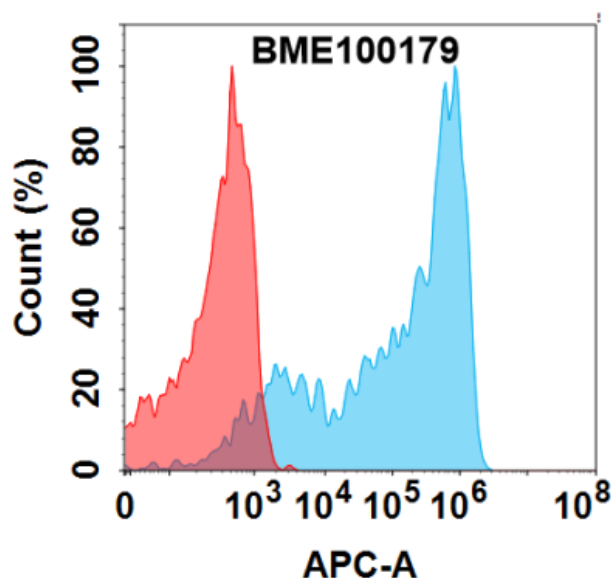
Figure 1. Flow cytometry analysis with 1 \mu g/mL TNF \alpha (golimumab biosimilar) mAb (28580) on Expi293 cells transfected with Human TNF \alpha protein (Blue histogram) or Expi293 transfected with irrelevant protein (Red histogram).
