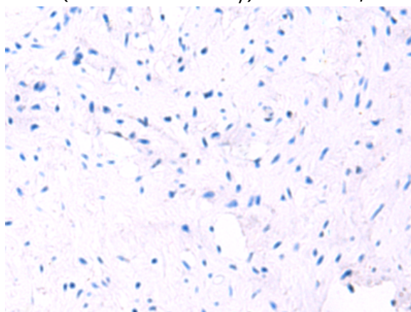
In comparison with the IHC on the left, the same paraffin-embedded Human cervical cancer tissue is first treated with fusion protein and then with D225857(Anti-RHAG Antibody) at dilution 1/130.
