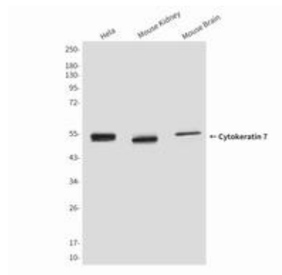
Western blot analysis of Cytokeratin 7 in HeLa, mouse Kidney, mouse Brain using Cytokeratin 7 antibody.
