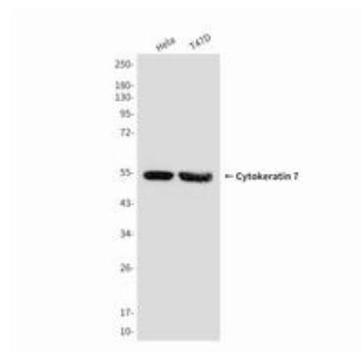
Western blot analysis of Cytokeratin 7 (9G9) in T47D and HeLa lysates using Cytokeratin 7 (9G9) antibody
