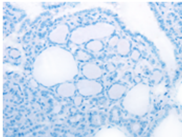
In comparison with the IHC on the left, the same paraffin-embedded Human thyroid cancer tissue is first treated with fusion protein and then with D220195(Anti-ADIPOR1 Antibody) at dilution 1/20.
