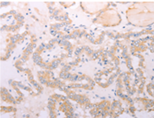
The image on the left is immunohistochemistry of paraffin-embedded Human thyroid cancer tissue using 216318(Anti-ADIPOR1 Antibody) at a dilution of 1/20.
