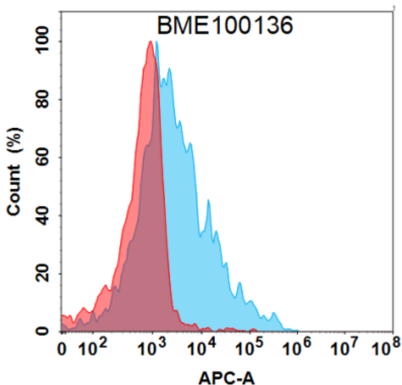
Figure 1. Flow cytometry analysis with 15 \mu\text{g}/\text{mL} APP (aducanumab biosimilar) mAb (28130) on Expi293 cells transfected with Human APP protein (Blue histogram) or Expi293 transfected with irrelevant protein (Red histogram).
