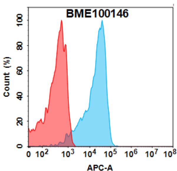
Figure 1. ITGAV protein is highly expressed on the surface of A549 cell membrane. Flow cytometry analysis with 1 µg/mL Anti-ITGAV(abituzumab biosimilar) mAb (28138) (Blue histogram) or isotype control mAb (Red histogram) on A549 cells.
