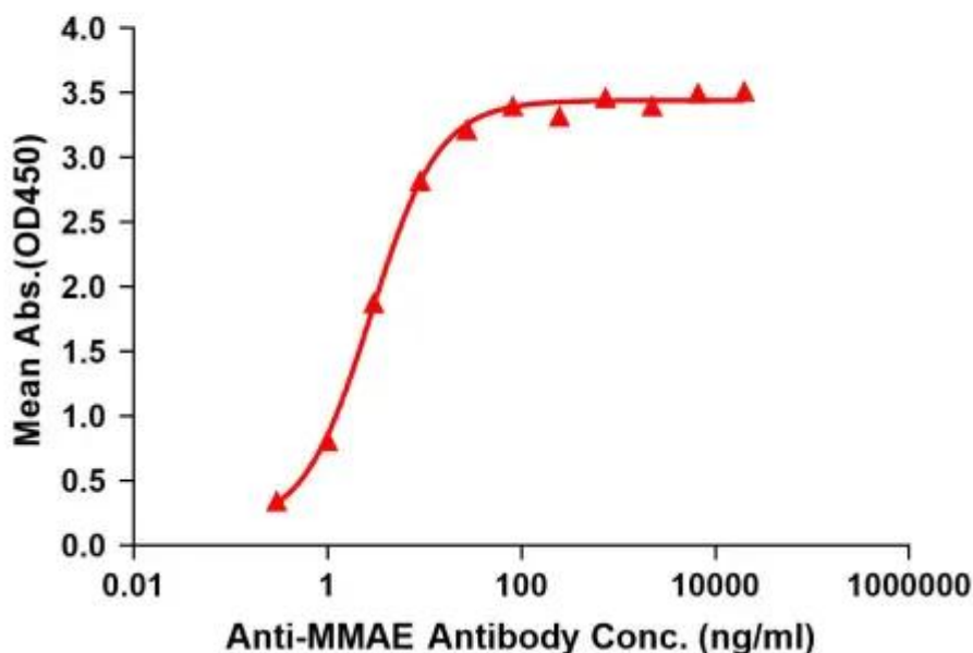
Figure 1. Elisa plates were pre-coated with IgG-MMAE (0.2 \mu g/per well). Serial diluted anti-MMAE monoclonal antibody (26101) solutions were added, washed, and incubated with secondary antibody before Elisa reading. From above data, the EC50 for anti-MMAE monoclonal antibody binding with IgG-MMAE is 2.820 ng/ml.
